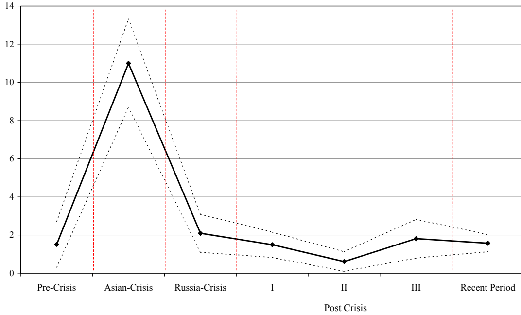
Chart 6. Estimated \beta Coefficient for Hutchison Whampoa Limited
